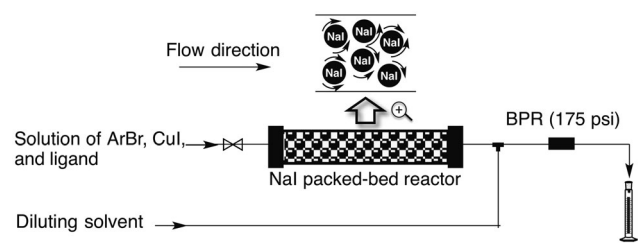
Figure 1. Experimental setup for the copper-catalyzed Finkelstein reaction of aromatics in flow. See the Supporting Information for details.
